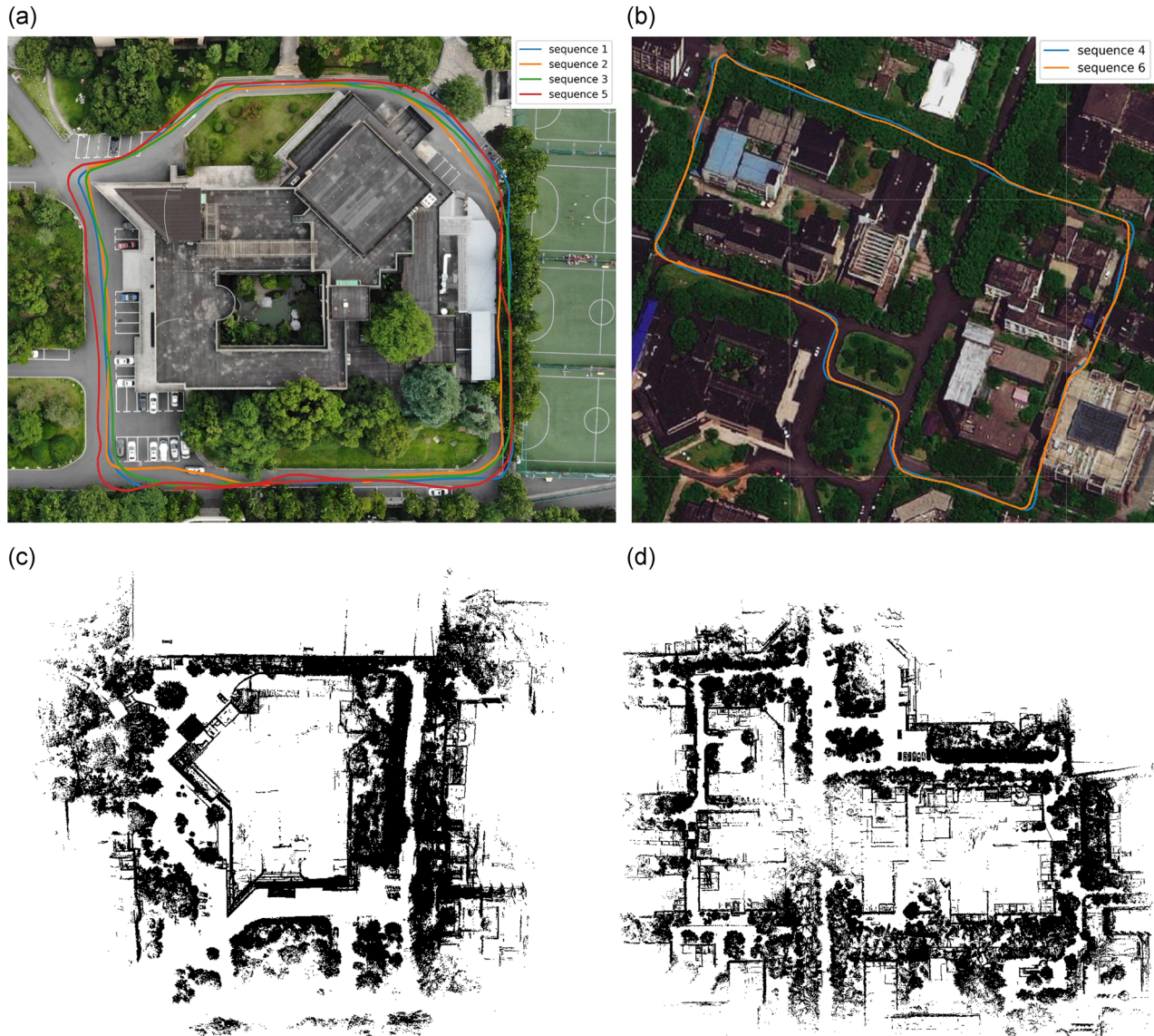
FIGURE 16 Bird's-eye views of our own data sets, including scene A and B, and the trajectories are also displayed. The prior LiDAR maps of both scenes are constructed on sequences 5 and 6. For clarity, we remove the ground points in both LiDAR maps. (a) A bird's-eye view of scene A; (b) A bird's-eye view of scene B; (c) Prior LiDAR map of scene A; and (d) Prior LiDAR map of scene B [Color figure can be viewed at wileyonlinelibrary.com ]
