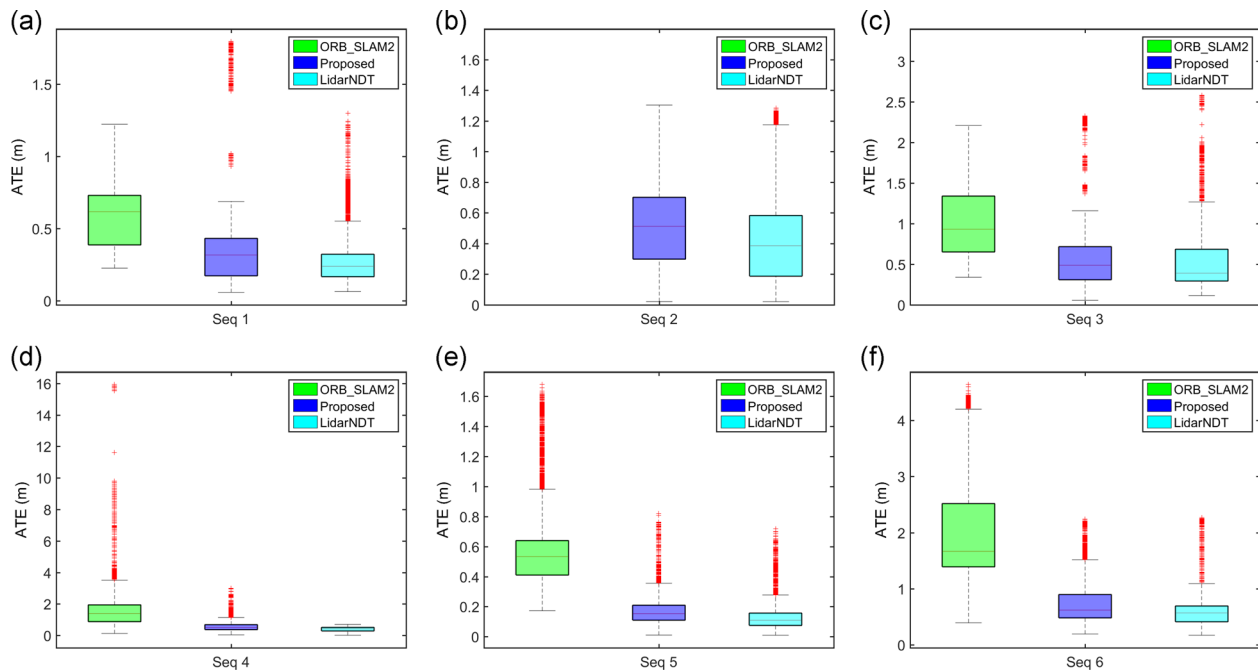
FIGURE 19 Norm of ATE, during the whole trajectory of one typical run, got from three types of map reuse system on our data set: the proposed online visual localization aided by prior LiDAR map ( Proposed ), the online visual localization aided by prior visual feature map ( ORB_SLAM2 ), the online LiDAR map aided by prior LiDAR map ( Lidar NDT ). As online visual localization aided by prior visual feature map fails on sequence 2, it's set blank. (a) On sequence 1; (b) On sequence 2; (c) On sequence 3; (d) On sequence 4; (e) On sequence 5; and (f) On sequence 6 [Color figure can be viewed at wileyonlinelibrary.com ]
