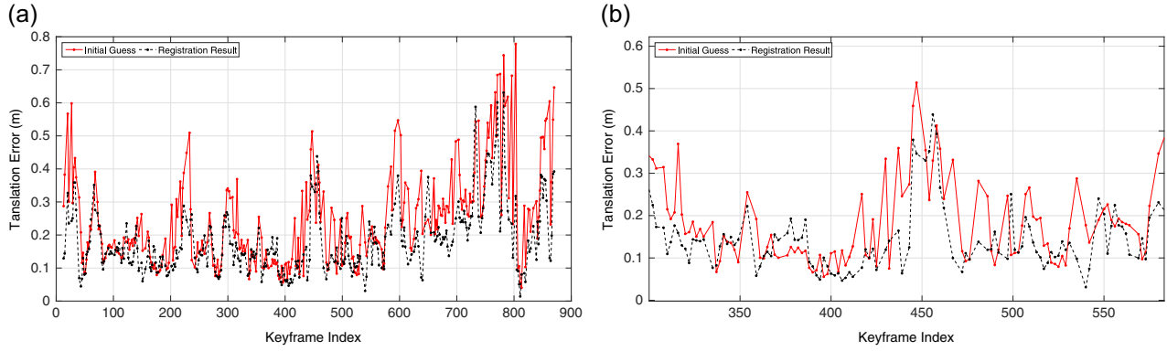
FIGURE 5 An example of the norm of absolute translation error before and after registration, which is performed on Sequence 05 of KITTI data set. (a) Norm of translation error; (b) A close view [Color figure can be viewed at wileyonlinelibrary.com ]
