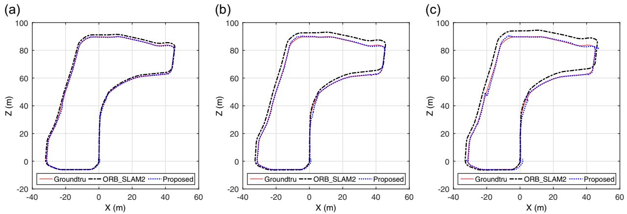
FIGURE 9 The trajectory estimated by the posed method and ORB-SLAM2 on Gazebo simulated data set under different disturbances. The red solid line indicates the trajectory of ground truth. Black dot-dash is estimated by ORB-SLAM2, and the blue dash is got from the proposed method. (a) On sequence with noise 5; (b) On sequence with noise 10; (c) On sequence with noise 15 [Color figure can be viewed at wileyonlinelibrary.com ]
