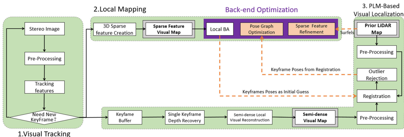
FIGURE 2 The proposed visual localization system with the PLM. The three main threads are visual tracking, local mapping, and PLM-based visual localization. Two types of visual maps are maintained: sparse feature visual map used for visual tracking and semidense visual map for registration. PLM, prior LiDAR map [Color figure can be viewed at wileyonlinelibrary.com ]
