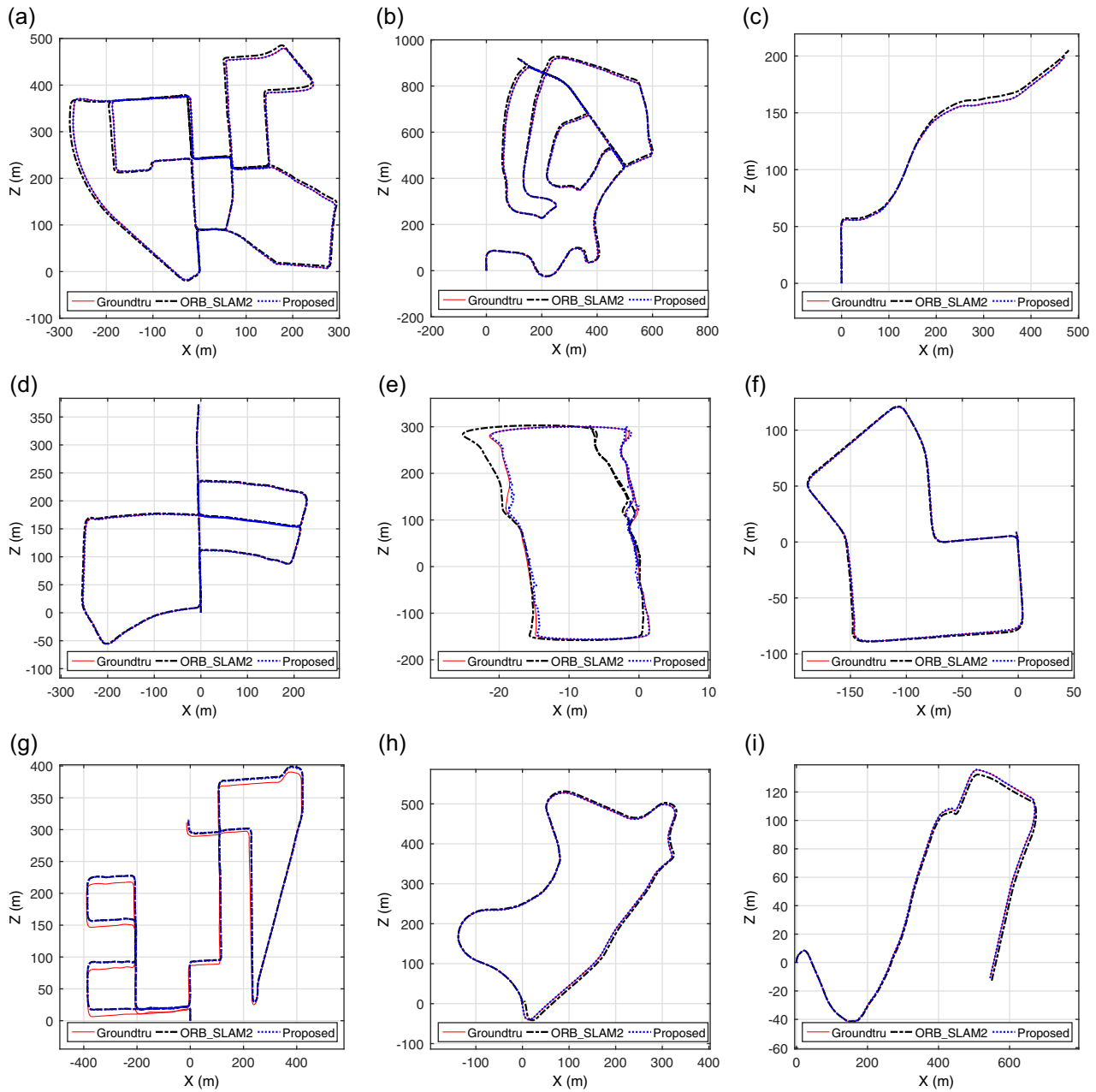
FIGURE 10 The estimated trajectories on some sequences of KITTl data set (Geiger et al., 2012). Red solid line indicates the trajectory of ground truth. Black dot-dash is estimated by ORB-SLAM2, and blue dash is got from our proposed method. (a) On sequence 00; (b) On sequence 02; (c) On sequence 03; (d) On sequence 05; (e) On sequence 06; (f) On sequence 07; (g) On sequence 08; (h) On sequence 09; and (i) On sequence 10 [Color figure can be viewed at wileyonlinelibrary.com ]
