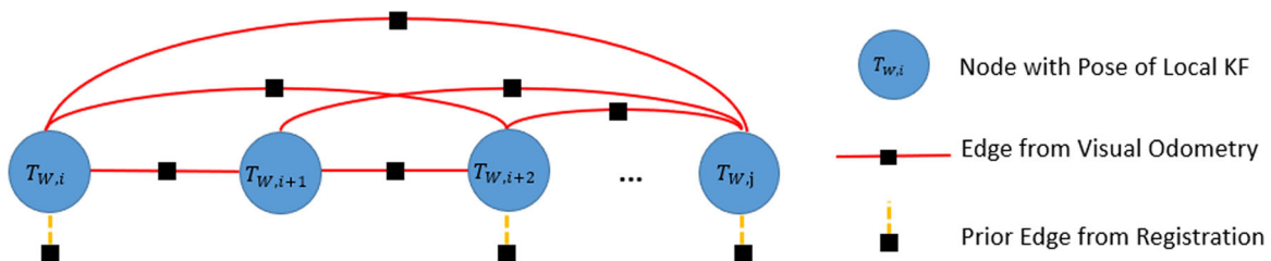
FIGURE 7 We construct the pose graph to fuse the registration and VO results. The blue circles represent the pose of the local keyframes. The red solid edges represent the relative-pose constraints from VO. The yellow dash edges denote the prior constraints obtained from ProW-NDT. VO, visual odometry [Color figure can be viewed at wileyonlinelibrary.com ]
