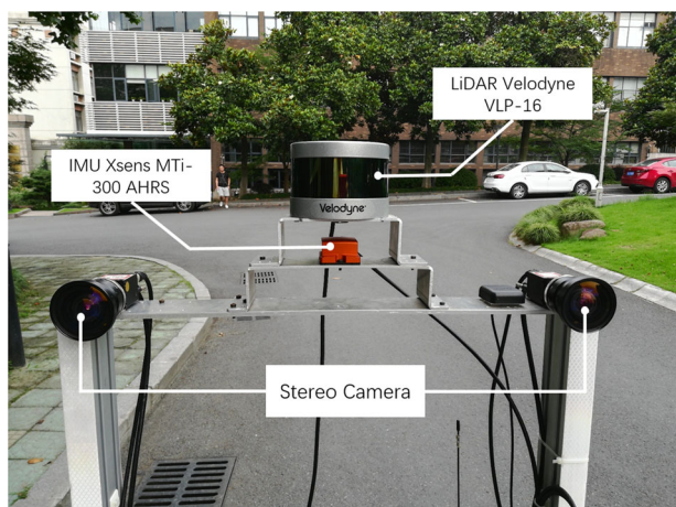
FIGURE 15 Sensors setup on our wheeled robot [Color figure can be viewed at wileyonlinelibrary.com ]
