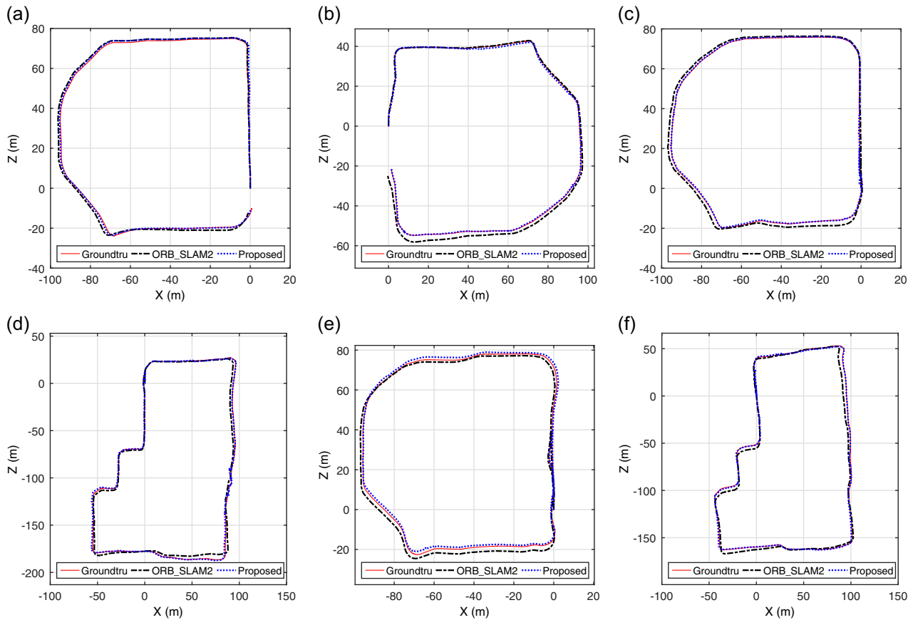
FIGURE 18 Trajectories estimated on our own data sets, shown in the camera frame. The proposed method is with the aid of in-run prior LiDAR map. Red solid line indicates the ground truth. Black dot-dash is estimated by ORB-SLAM2, and the blue dash is got from our proposed method. (a) On sequence 1; (b) On sequence 2; (c) On sequence 3; (d) On sequence 4; (e) On sequence 5; and (f) On sequence 6 [Color figure can be viewed at wileyonlinelibrary.com ]
