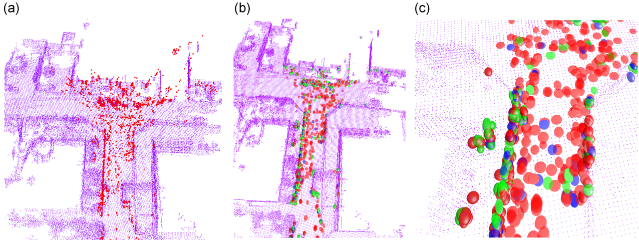
FIGURE 6 Surfels are extracted around sparse visual features from the prior LiDAR map. They are used to correct the positions of the 3D Visual features. Extracted surfels are color-coded by normal directions (a) Sparse visual features in LiDAR map; (b) Surfels from the prior LiDAR map; (c) A close view of the extracted surfels [Color figure can be viewed at wileyonlinelibrary.com ]
