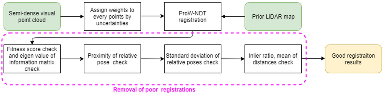
FIGURE 4 Flow chart of registration. Points in the semidense visual point cloud are assigned with different weights by uncertainties (see Equation (13)); Then the point cloud registered with the prior LiDAR map; The poor registration results will be removed by designed criteria described in Section 4.2.1. Only the good registration results will be used in the later pose graph optimization [Color figure can be viewed at wileyonlinelibrary.com ]
