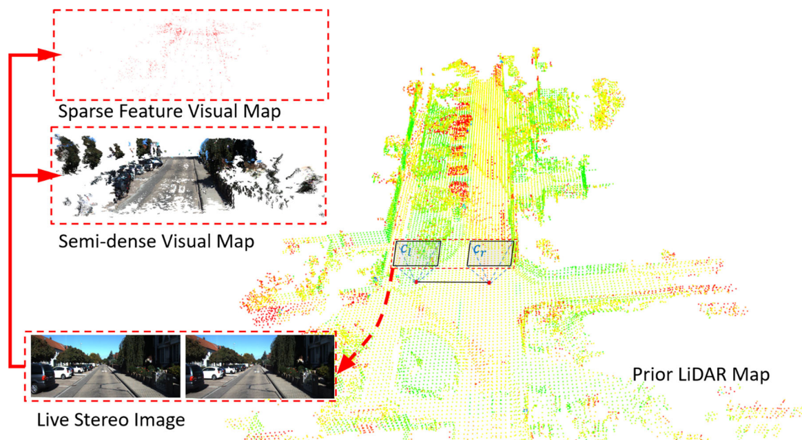
FIGURE 1 We propose a stereo visual localization system aided by a prior LiDAR map. In this system, both the sparse feature visual map and semidense visual map are constructed in order for robust fusion with the prior LiDAR map to provide low-cost, high-precision localization solutions [Color figure can be viewed at wileyonlinelibrary.com ]
