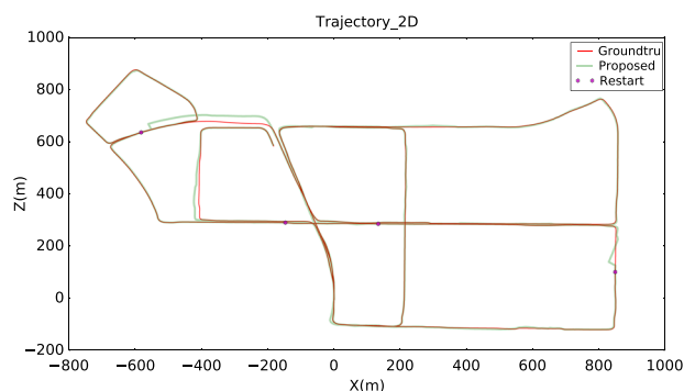
FIGURE 14 The trajectory estimates (in green) on the whole Urban 28 sequence (11.47 km) and the ground truth (in red). There are in total four restarts along the whole trajectory. The restart positions are marked by magenta hexagon [Color figure can be viewed at wileyonlinelibrary.com ]
