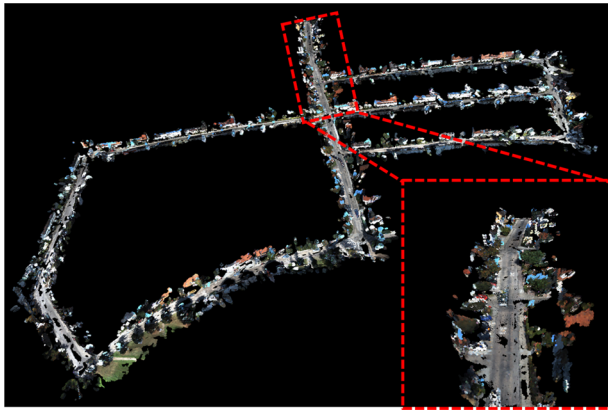
FIGURE 11 A global semidense visual map on sequence 05 of KITTI data set [Color figure can be viewed at wileyonlinelibrary.com ]
