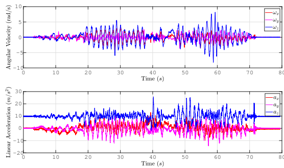
Fig. 6: Raw IMU measurements over the high-dynamic Indoor-C sequence.
