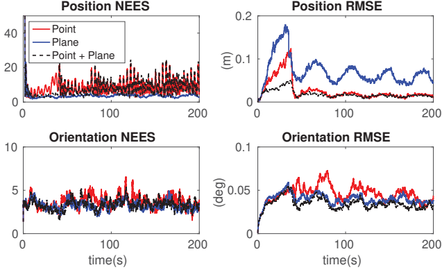
Fig. 1: Simulation results: Averaged NEES and RMSE values of the IMU poses (orientation and position) of the proposed aided INS with point and/or plane features.
