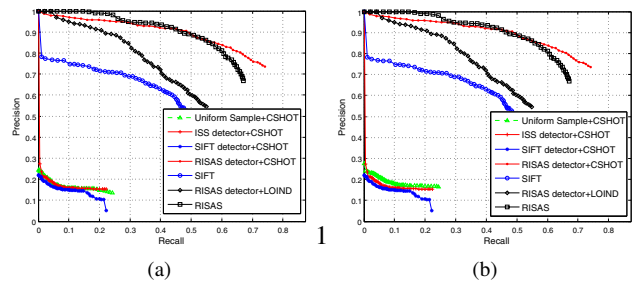
Fig. 15: Precision-Recall curves corresponding to Fig. 14.
