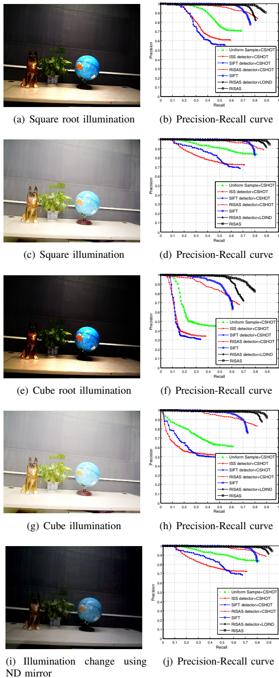
Fig. 11: RISAS evaluation under illumination variations.
