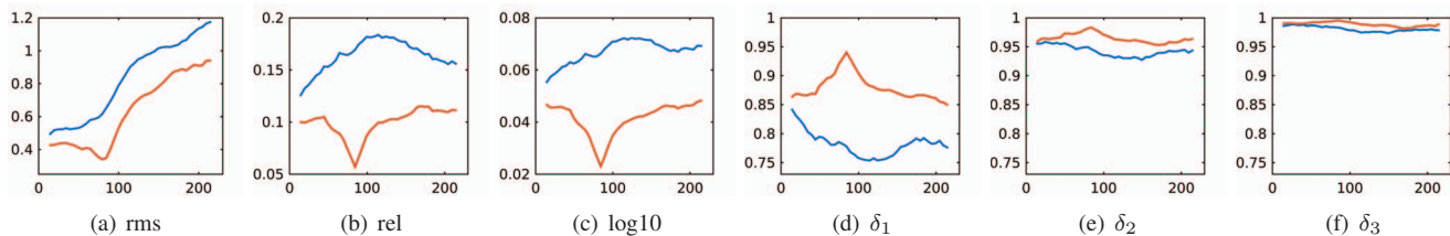
Fig. 6. Results evaluated at different heights of the test images in NYUD2. In each figure, the x-axis is the height with respect to the ground in centimeter, and the y-axis is the evaluation metric. The blue line denotes the performance of the depth estimation with only RGB image, and the red line denotes the performance of the depth estimation with combination of the RGB image and a single line of laser range scan with height at 80cm. Best viewed in color.
